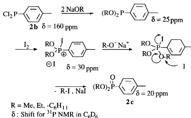
Scheme 2 : Suggested mechanism for tolyldichlorophosphine oxidation by iodine
